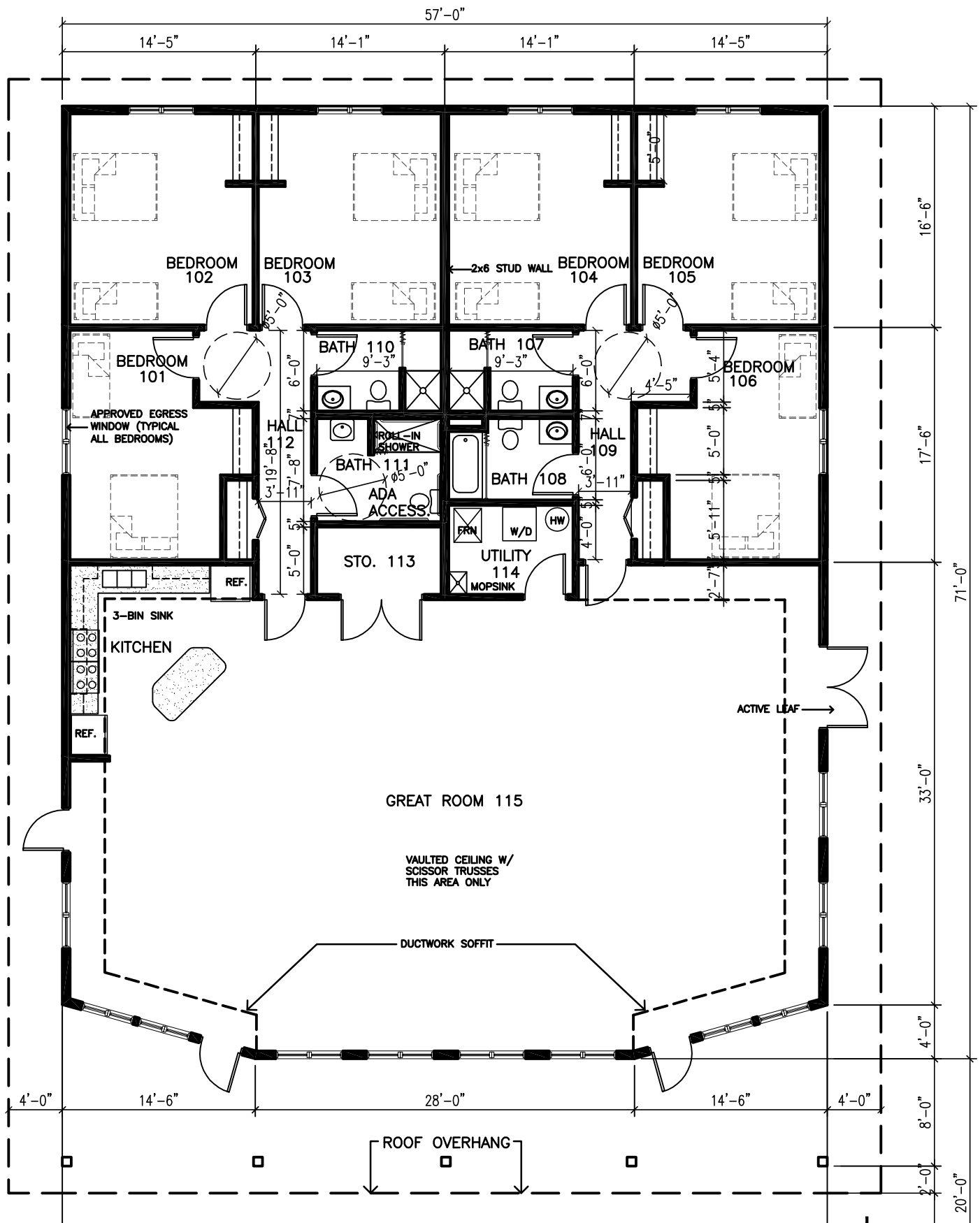
FLOORPLAN SCALE 1" = 10'-0"
